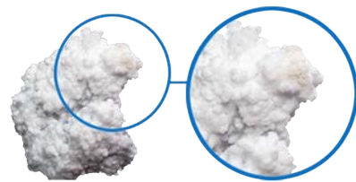
Aragonit (nachher)
